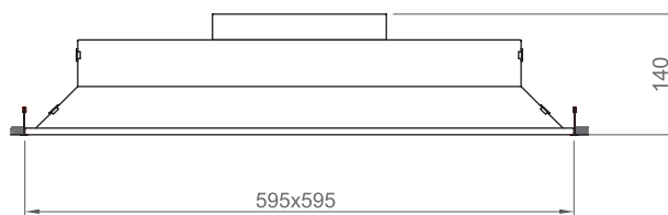
Ceiling Type-Cut-out
